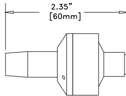
1/8" NPT (HPM-2002s-01)
