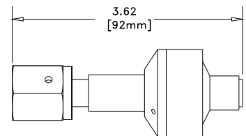
1/2" VCR (HPM-2002s-08)
