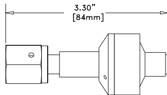
1/4" VCR (HPM-2002s-02)
